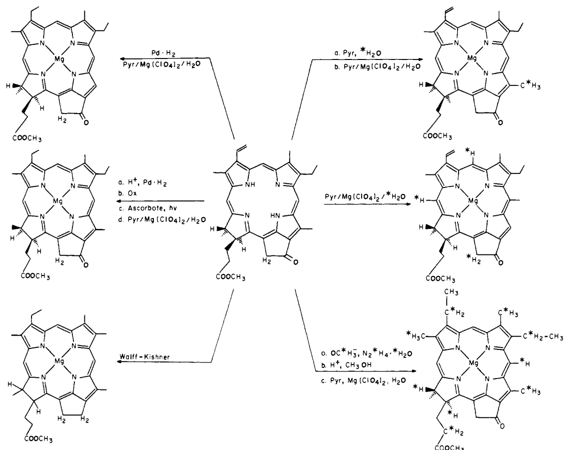
Chart II. Reaction Scheme for Selective Deuteration and Derivative Preparations from Methylpyropheophorbide a (2)
